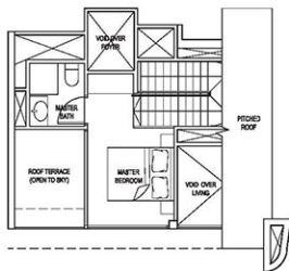
UPPER FLOOR
