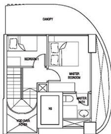
UPPER FLOOR
