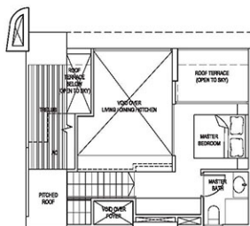
UPPER FLOOR
