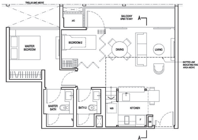
TYPE C2c 91 sqm / 980 sq ft. (including void area of 21 sqm/226 sq ft. above living, dining and kitchen) #10-05
