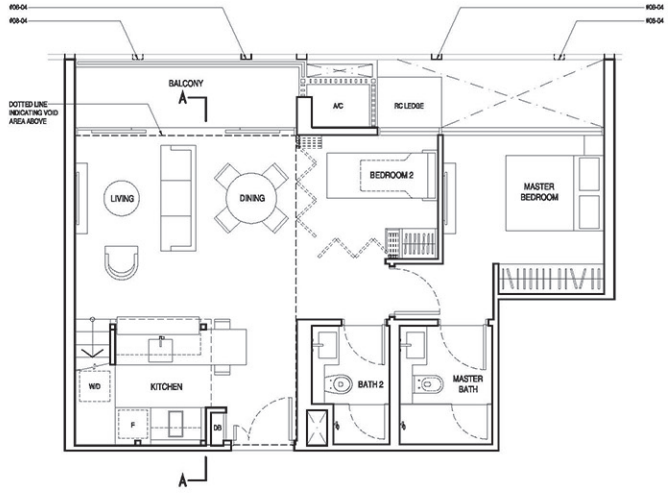
TYPE C1a 97 sq.m. / 1,044 sq.ft. (including void area of 29 sq.m./312 sq.ft. above living, dining and kitchen) #05-04 #03-04
