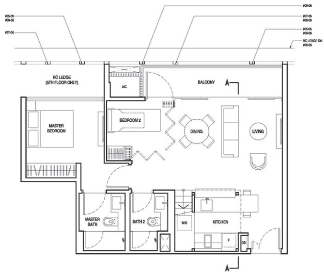
TYPE C2b 70 sq.m. / 753 sq.ft. R05-05 R07-05 R09-05
