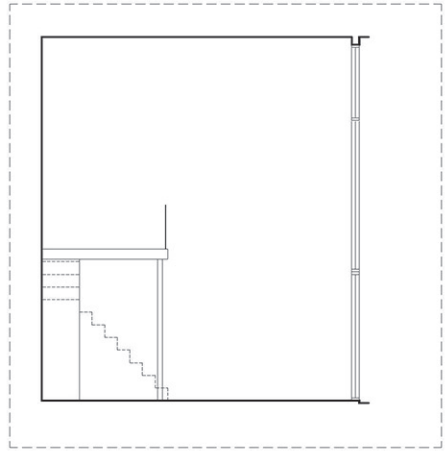
PART SECTION A-A FLOOR TO FLOOR 7.20 m. ABOVE LIVING/ DINING AND KITCHEN
